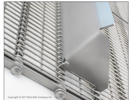
Solid stainless steel flight
